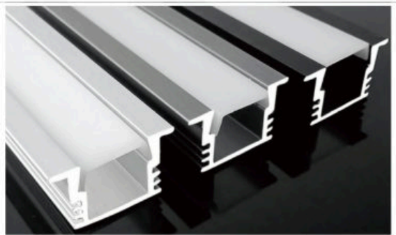
GD-015 Finish: Silver Diffuser: Clear / Opal / Frost / Black
