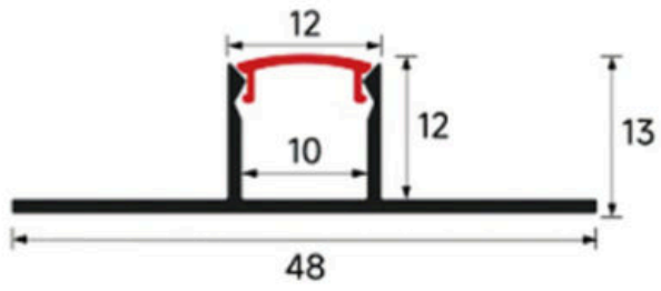
LSH-1313DD Double-wing plaster-in Cover & finish: Confirm by model
