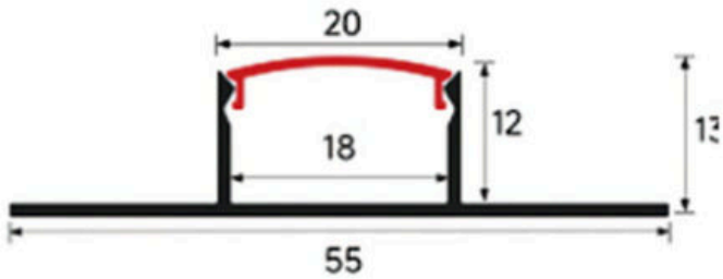
LSH-2013DD Double-wing plaster-in Cover & finish: Confirm by model
