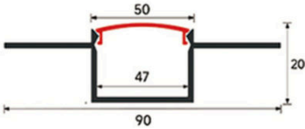
LSH-5020DU Double-wing plaster-in Cover & finish: Confirm by model
