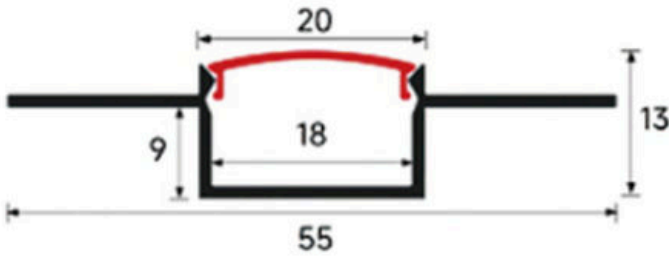
LSH-2013DU Double-wing plaster-in Cover & finish: Confirm by model
