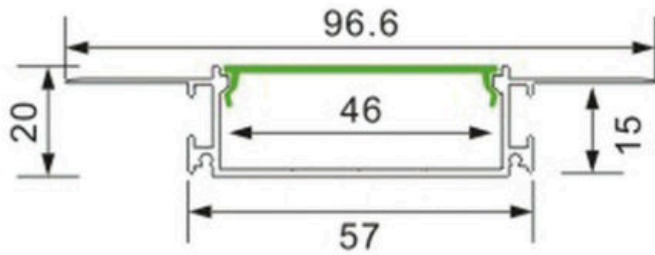
XT-381 Color: Black / White / Silver PC Cover: Opal / Frost
