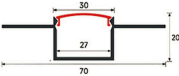
LSH-3020DD Double-wing plaster-in Cover & finish: Confirm by model
