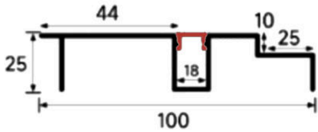
LSH-100 Double-Step Double-step ceiling profile Diffuser: PC cover
