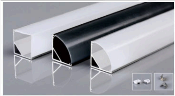
LSH58 16×16mm Color: Black/White/Silver Diffuser Cover: Clear/Frost/Opal/Black
