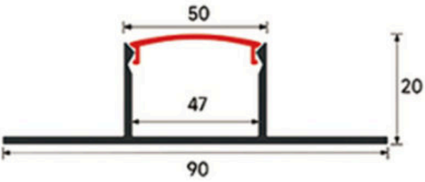
LSH-5020DD Double-wing plaster-in Cover & finish: Confirm by model
