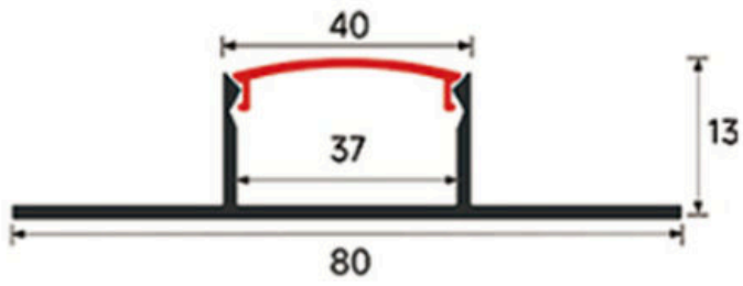
LSH-4013DD Double-wing plaster-in Cover & finish: Confirm by model
