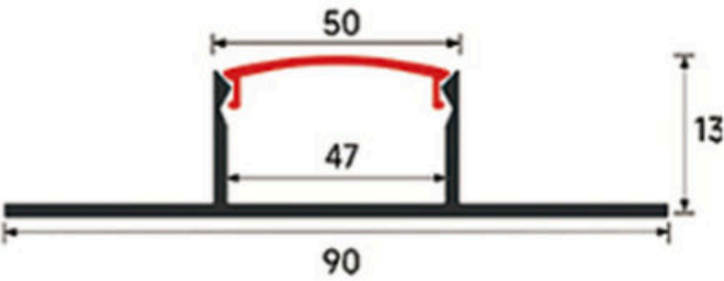
LSH-5013DD Double-wing plaster-in Cover & finish: Confirm by model
