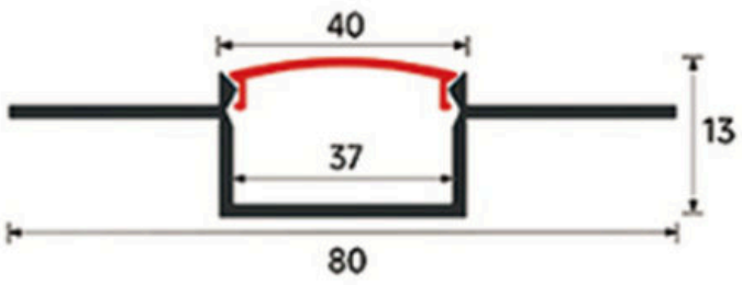
LSH-4013DU Double-wing plaster-in Cover & finish: Confirm by model
