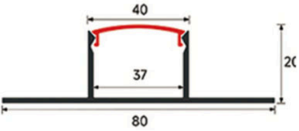
LSH-4020DD Double-wing plaster-in Cover & finish: Confirm by model
