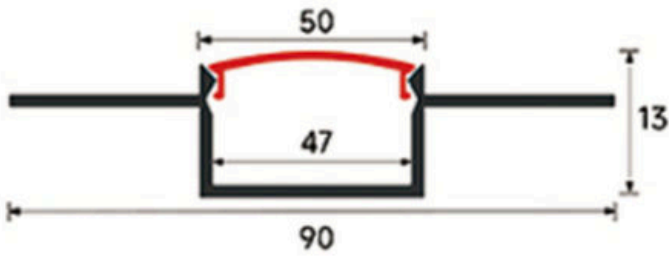
LSH-5013DU Double-wing plaster-in Cover & finish: Confirm by model
