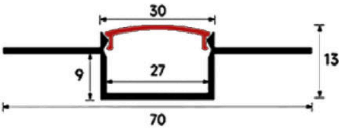
LSH-3013DU Double-wing plaster-in Cover & finish: Confirm by model
