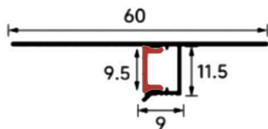
LSH-6014 Upper Flange
