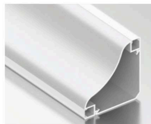
LSH-6969 Dual-channel cornice profile Diffuser: PC cover
