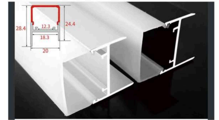
GD-011 Color: Black / White / Silver PC Cover: Opal / Frost
