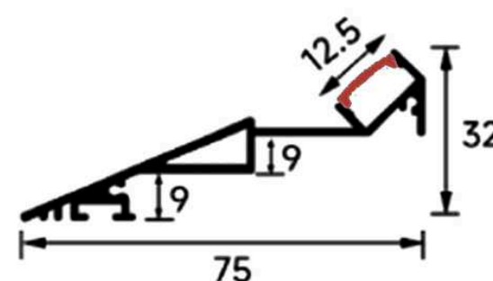
LSH-7532 Slim Flange
