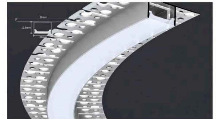
LSH-2018DW 20×18mm Color: Black / White / Silver Silicone Cover: Clear / Frost / Opal / Black
