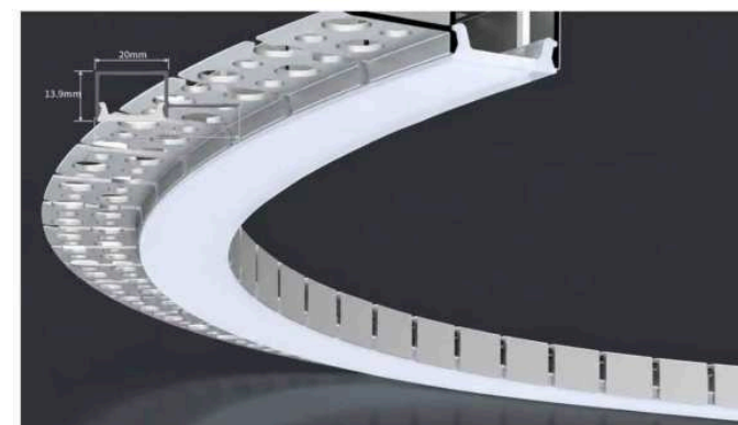
LSH-2018SWL 20×18mm Color: Black / White / Silver Silicone Cover: Clear / Frost / Opal / Black
