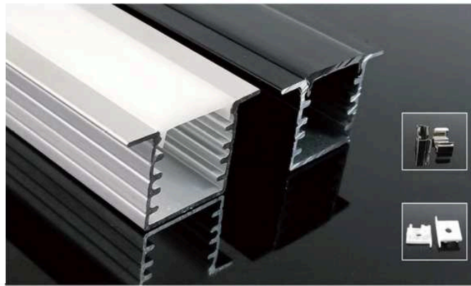
XT-375 Finish: Silver Diffuser: Clear / Opal / Frost / Black
