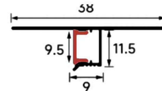
LSH-3814 Upper Flange
