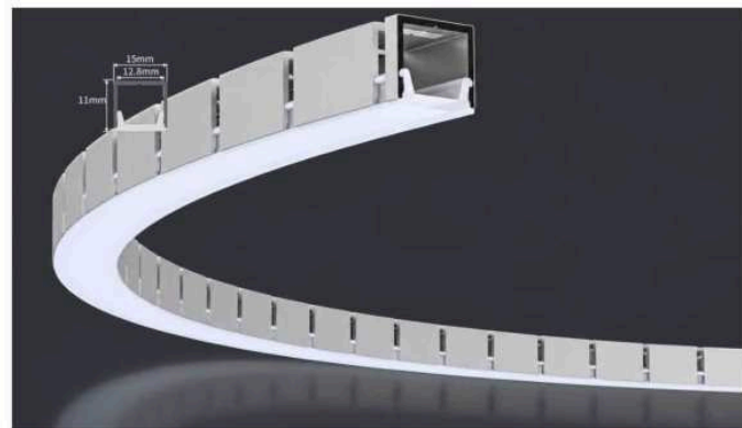
LSH-1513NW 15×13mm Color: Black / White / Silver Silicone Cover: Clear / Frost / Opal / Black
