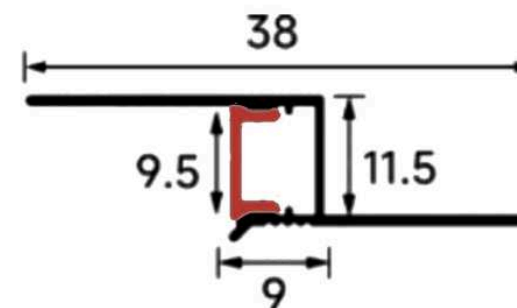
LSH-3814 Lower Flange
