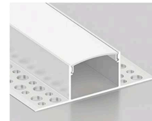
LSH-4020DD Double-wing plaster-in Cover & finish: Confirm by model
