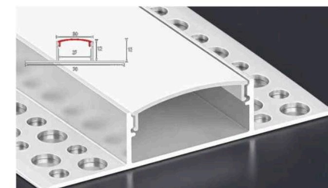
LSH-3013DD Double-wing plaster-in Cover & finish: Confirm by model
