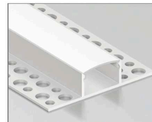
LSH-2013DD Double-wing plaster-in Cover & finish: Confirm by model
