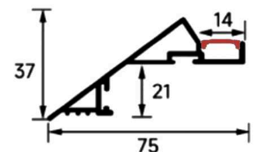
LSH-7537 Slim Flange
