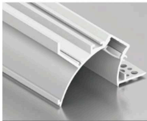
LSH-075 Cove lighting profile Diffuser: PC cover
