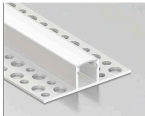
LSH-1313DD Double-wing plaster-in Cover & finish: Confirm by model
