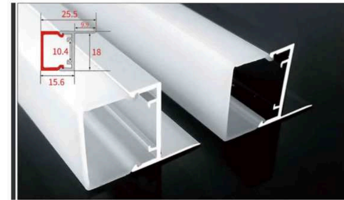
GD-010 Color: Black / White / Silver PC Cover: Opal / Frost
