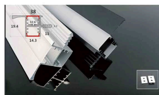
KK-029 Finish: Silver Diffuser: Clear / Opal / Frost / Black
