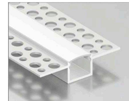
LSH-1513DU Double-wing plaster-in Cover & finish: Confirm by model
