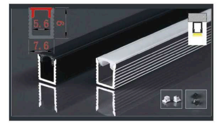
XT-231 Narrow Ribbed Channel Drawing: SDXT-231; prefix to verify
