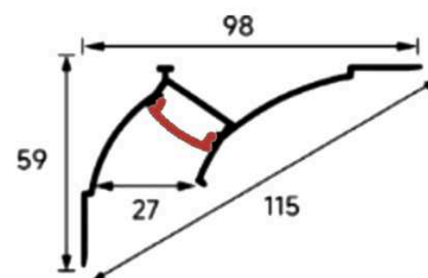
LSH-068 Large / Thick Wall
