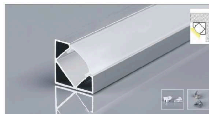
LSH59 18×18mm Color: Black/White/Silver Diffuser Cover: Clear/Frost/Opal/Black
