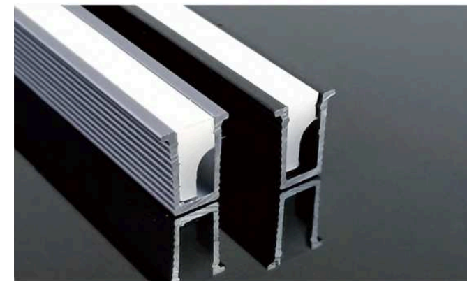
GD-004 Finish: Silver Diffuser: Clear / Opal / Frost / Black
