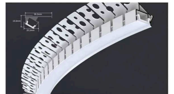
LSH-2018XWL 20×18mm Color: Black / White / Silver Silicone Cover: Clear / Frost / Opal / Black
