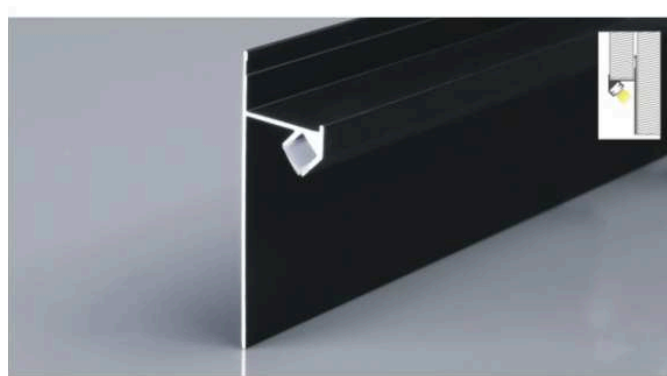
XT-47B Color: Black / White / Silver PC Cover: Opal / Frost
