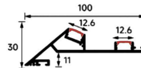
LSH-10030 Slim Flange
