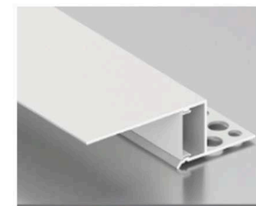
LSH-7021 Lower Flange Ceiling edge profile Diffuser: PC cover
