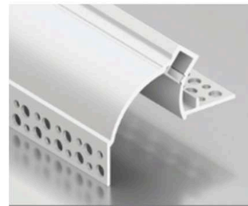
LSH-076 Cove lighting profile Diffuser: PC cover
