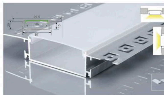
XT-381 Color: Black / White / Silver PC Cover: Opal / Frost
