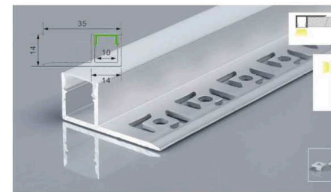
XT-283 Color: Black / White / Silver PC Cover: Opal / Frost
