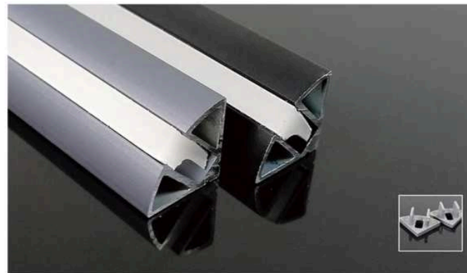
LSH006 13×13mm Color: Black/White/Silver Diffuser Cover: Clear/Frost/Opal/Black
