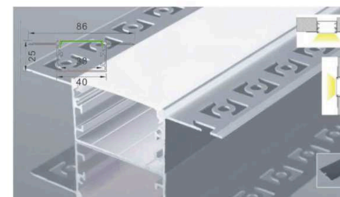
XT-563 Color: Black / White / Silver PC Cover: Opal / Frost
