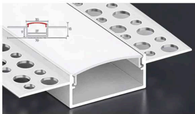
LSH-3013DU Double-wing plaster-in Cover & finish: Confirm by model
