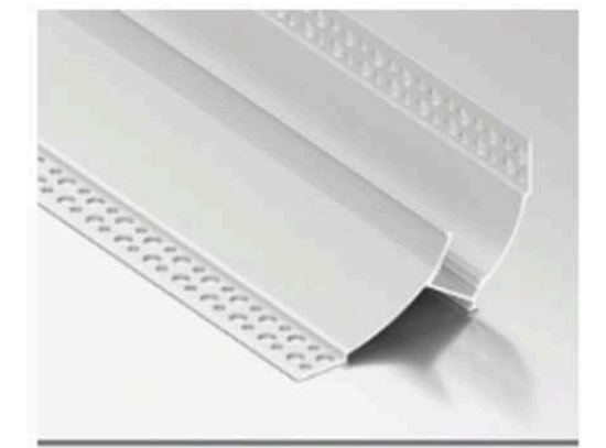
LSH-068 Medium Cove lighting profile Diffuser: PC cover
