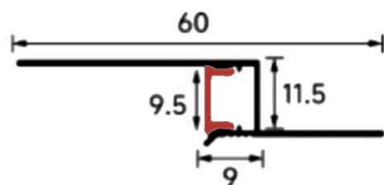
LSH-6014 Lower Flange
