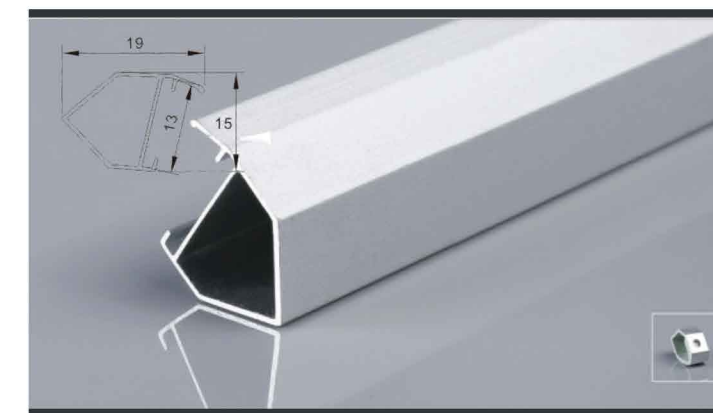
SDXT-61 Color: Black / White / Silver PC Cover: Opal / Frost
