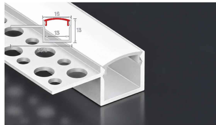
LSH-1513SU Single-wing plaster-in Cover & finish: Confirm by model
