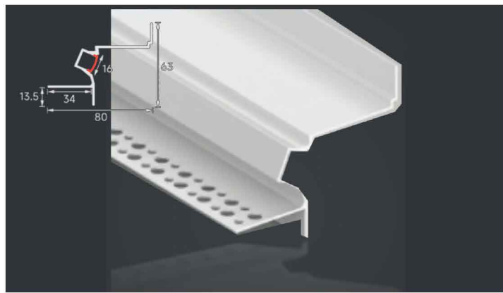
LSH-7962 Cove lighting profile Diffuser: PC cover
