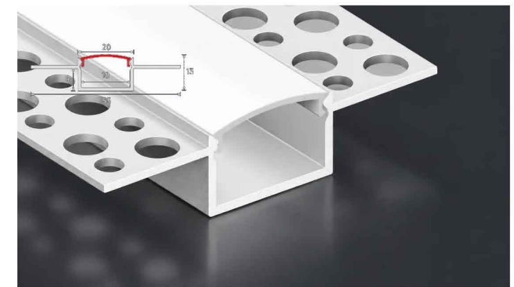
LSH-2013DU Double-wing plaster-in Cover & finish: Confirm by model
