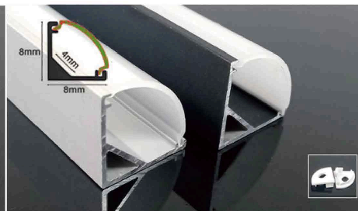
LSH56 8x8mm Color: Black/White/Silver Diffuser Cover: Clear/Frost/Opal/Black
