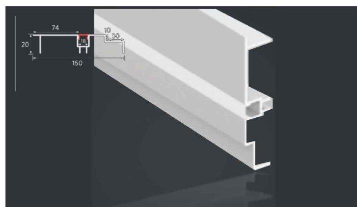
LSH-150 Double-Step Double-step ceiling profile Diffuser: PC cover
