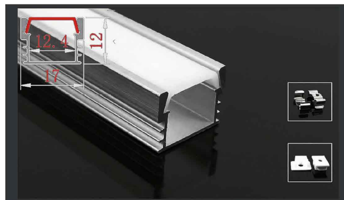
XT-211 Compact Rectangular Channel Cover & finish: Specify with order
