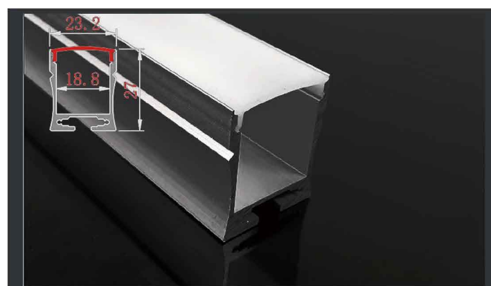
XT-339 Stepped Linear Housing Cover & finish: Specify with order
