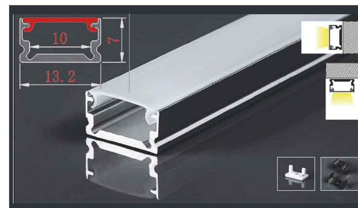
SDXT-30 Slim Strip Channel Cover & finish: Specify with order
