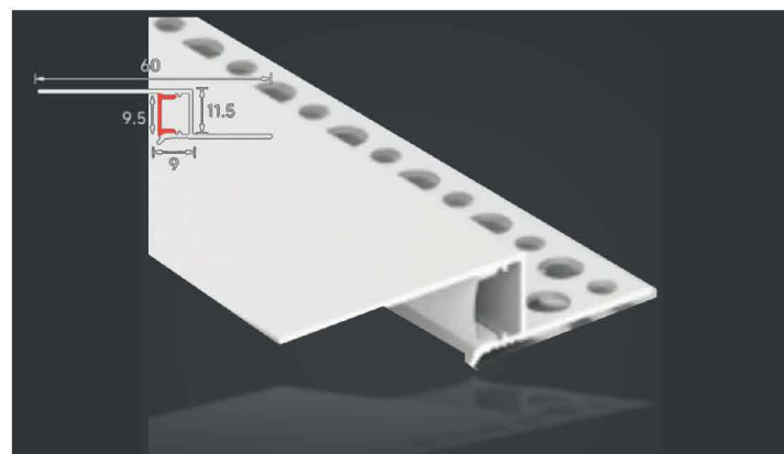
LSH-6014 Lower Flange Ceiling edge profile Diffuser: PC cover
