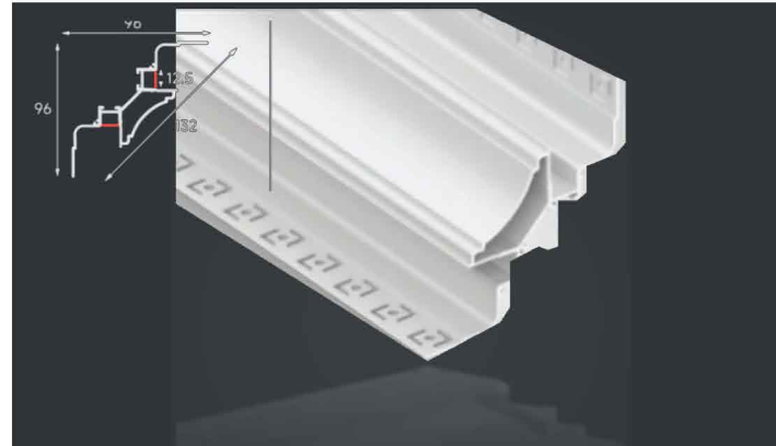
LSH-9595 Dual-channel cornice profile Diffuser: PC cover
