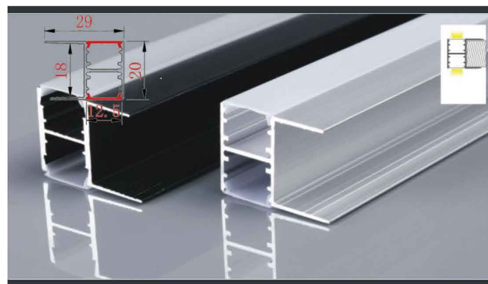
SDXT-345 Color: Black / White / Silver PC Cover: Opal / Frost
