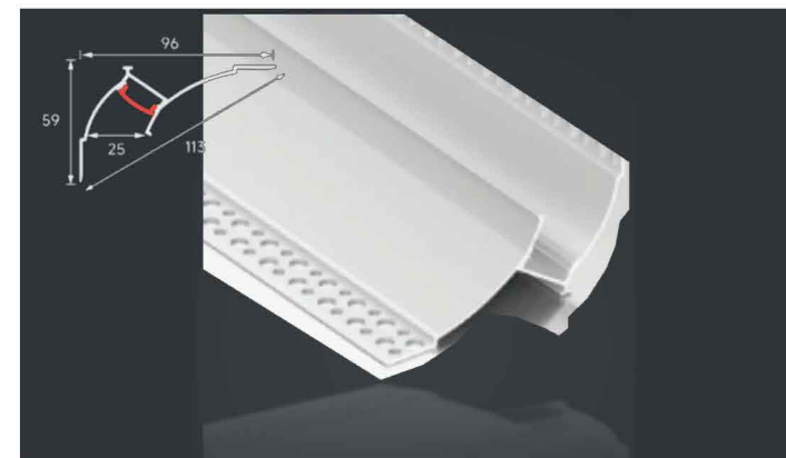
LSH-068 Large / Thin Wall Cove lighting profile Diffuser: PC cover
