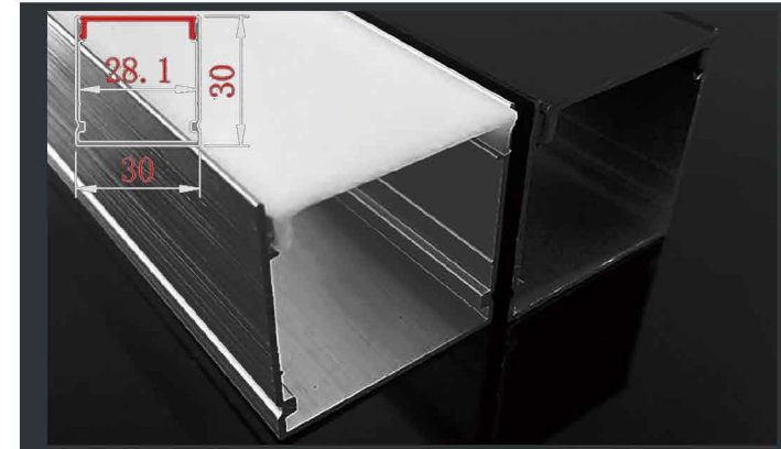
XT-371 Square Linear Housing Cover & finish: Specify with order
