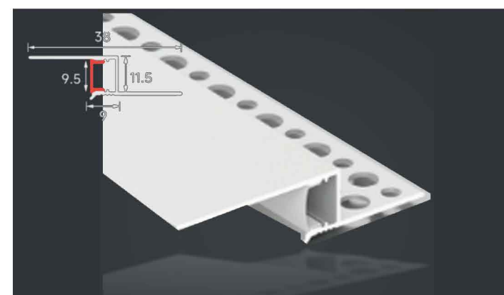
LSH-3814 Lower Flange Ceiling edge profile Diffuser: PC cover
