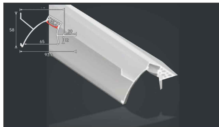
LSH-075B Cove lighting profile Diffuser: PC cover
