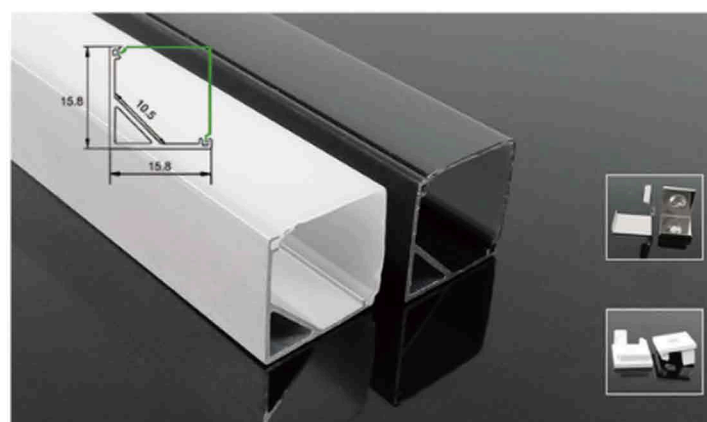
LSH58B 16x16mm Color: Black/White/Silver Diffuser Cover: Clear/Frost/Opal/Black
