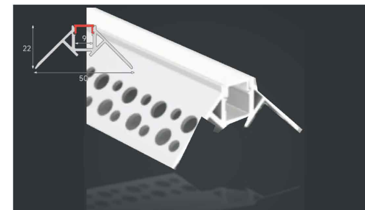
LSH-646 Plaster-in corner profile Diffuser: PC cover
