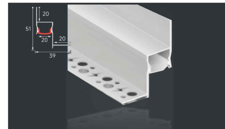
LSH-078 Ceiling edge profile Diffuser: PC cover
