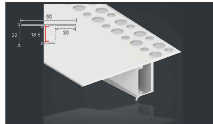
LSH-5020 Upper Flange Ceiling edge profile Diffuser: PC cover
