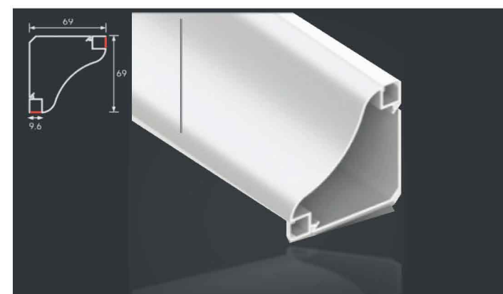
LSH-6969 Dual-channel cornice profile Diffuser: PC cover
