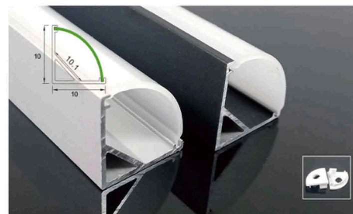
LSH57 10x10mm Color: Black/White/Silver Diffuser Cover: Clear/Frost/Opal/Black
