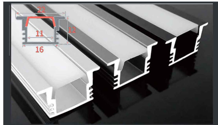
GD-015 Finish: Silver Diffuser: Clear / Opal / Frost / Black
