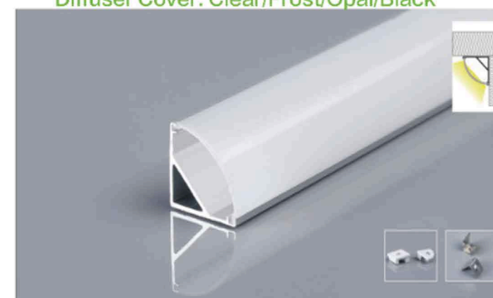
LSH407 13x13mm Color: Black/White/Silver Diffuser Cover: Clear/Frost/Opal/Black
