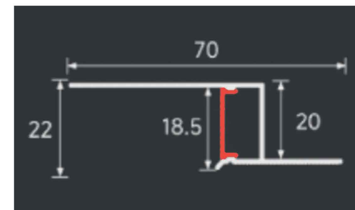
LSH-7021 Lower Flange
