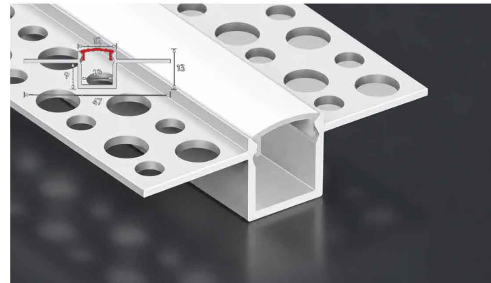
LSH-1313DU Double-wing plaster-in Cover & finish: Confirm by model
