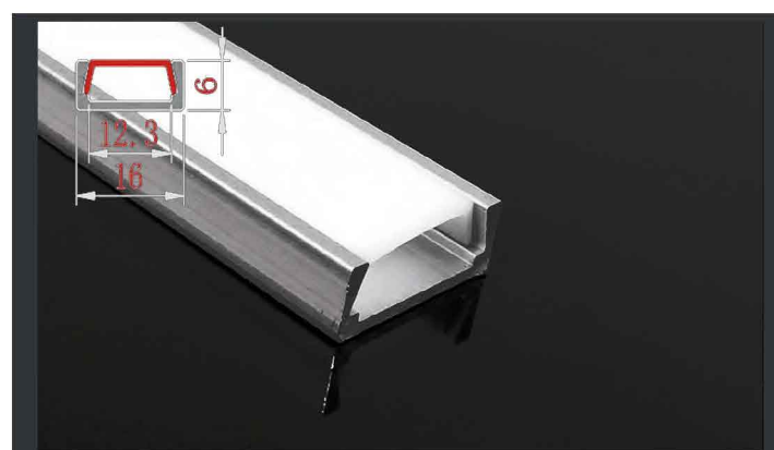
XT-200 Mini Shallow Channel Cover & finish: Specify with order
