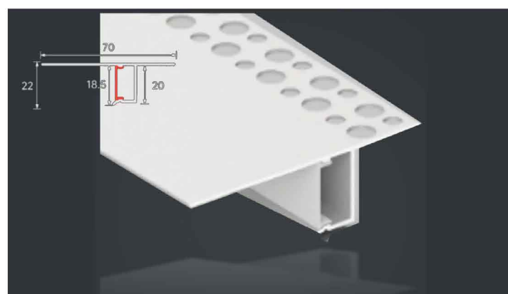
LSH-7021 Upper Flange Ceiling edge profile Diffuser: PC cover
