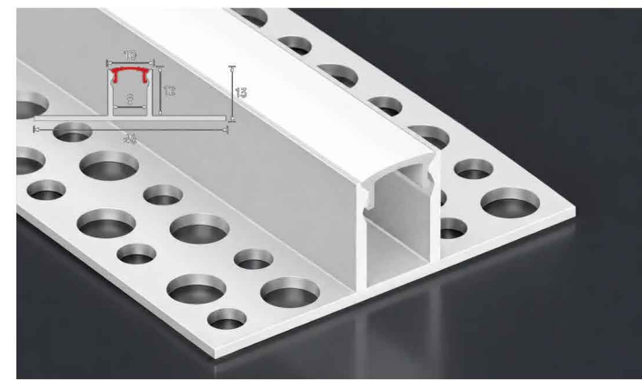
LSH-1013DD Double-wing plaster-in Cover & finish: Confirm by model
