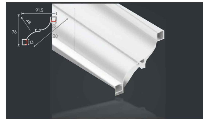
LSH-8080 Dual-channel cornice profile Diffuser: PC cover
