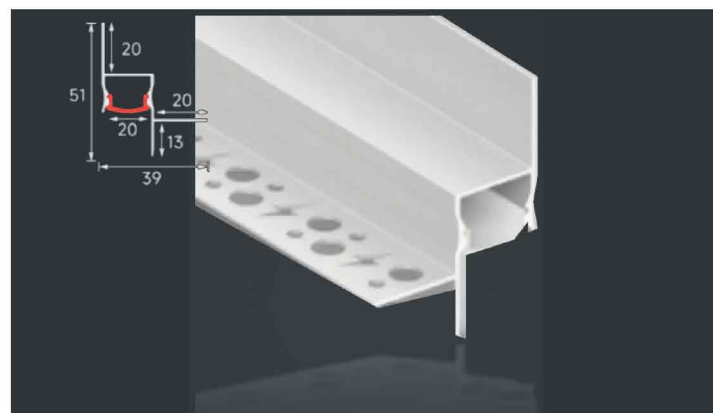
LSH-078A Ceiling edge profile Diffuser: PC cover
