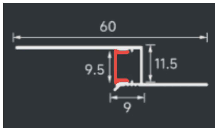
LSH-6014 Lower Flange
