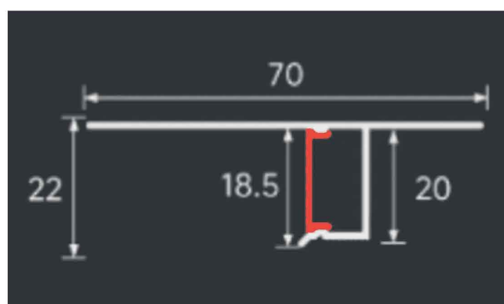
LSH-7021 Upper Flange
