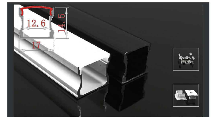
XT-57 Compact Strip Channel Cover & finish: Specify with order
