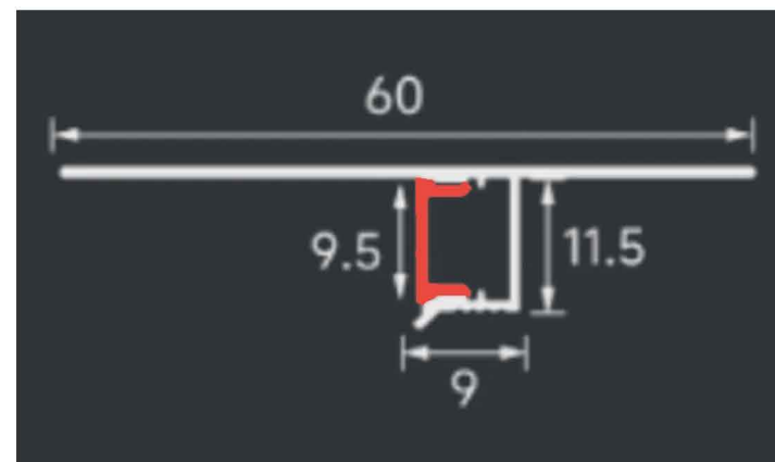
LSH-6014 Upper Flange
