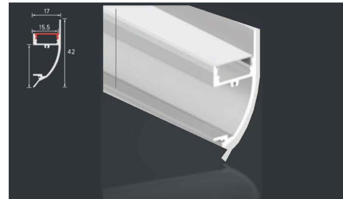
LSH-066 Cove lighting profile Diffuser: PC cover
