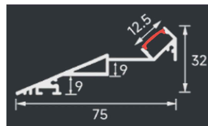
LSH-7532 Slim Flange
