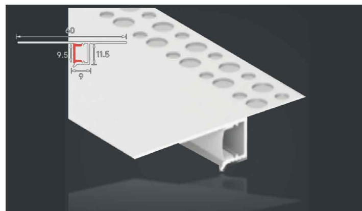
LSH-6014 Upper Flange Ceiling edge profile Diffuser: PC cover
