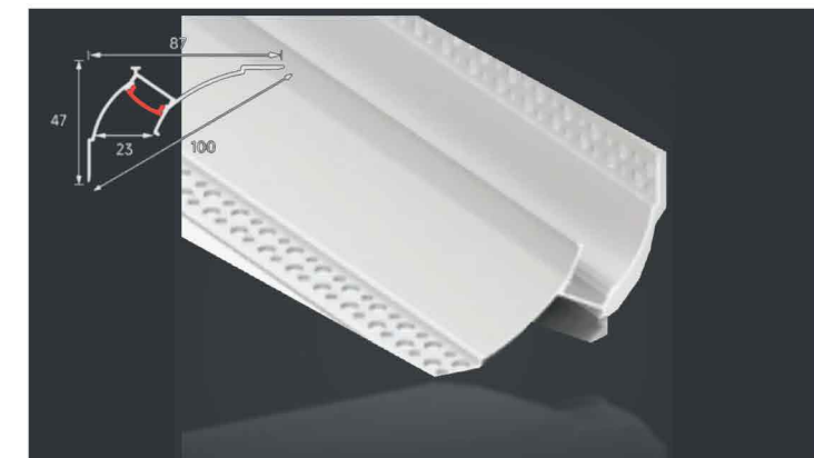
LSH-068 Medium Cove lighting profile Diffuser: PC cover
