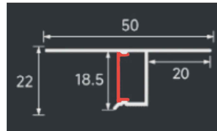
LSH-5020 Upper Flange
