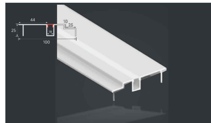
LSH-100 Double-Step Double-step ceiling profile Diffuser: PC cover
