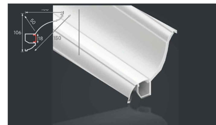
LSH-149 Cornice / wall junction profile Diffuser: PC cover
