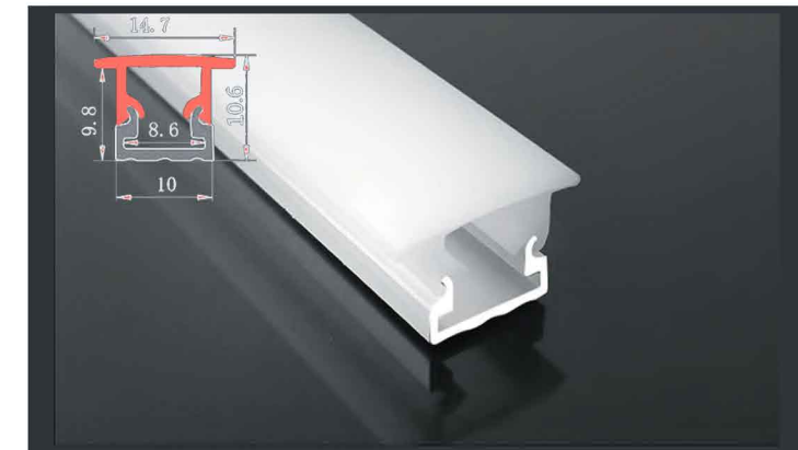
GD-024 Finish: Silver Diffuser: Clear / Opal / Frost / Black
