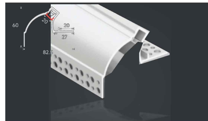
LSH-076 Cove lighting profile Diffuser: PC cover
