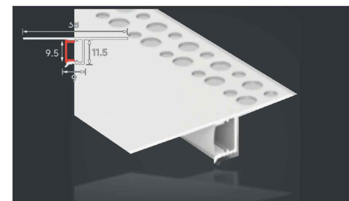
LSH-3814 Upper Flange Ceiling edge profile Diffuser: PC cover
