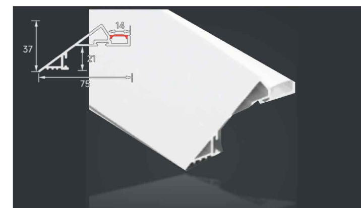
LSH-7537 Slim Flange Angled cove lighting profile Diffuser: PC cover
