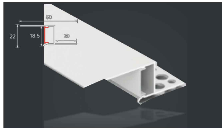
LSH-5020 Lower Flange Ceiling edge profile Diffuser: PC cover
