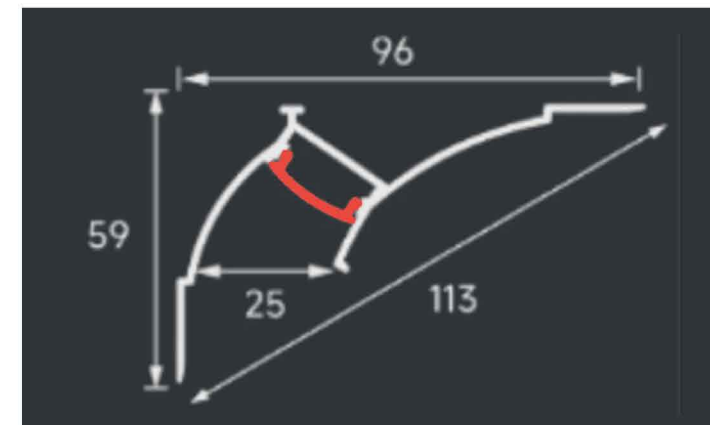
LSH-068 Large / Thin Wall
