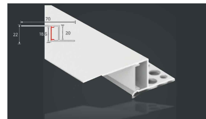
LSH-7021 Lower Flange Ceiling edge profile Diffuser: PC cover
