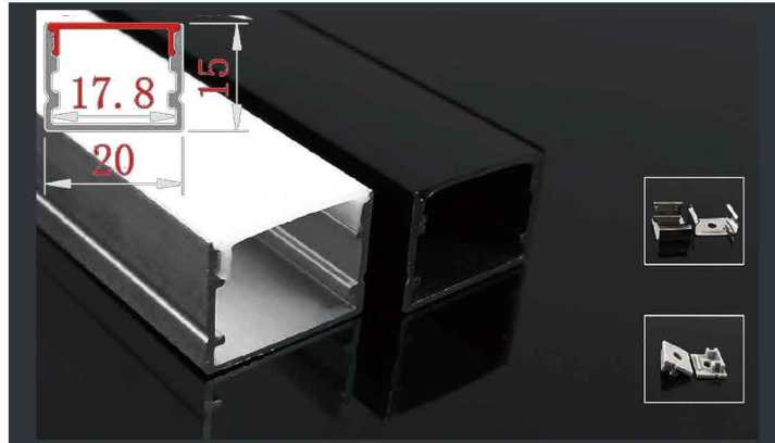
XT-369 Compact Rectangular Channel Cover & finish: Specify with order
