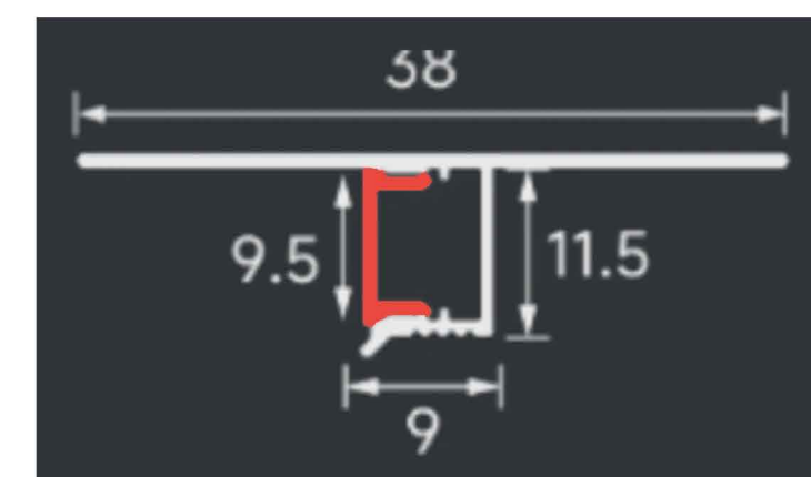
LSH-3814 Upper Flange
