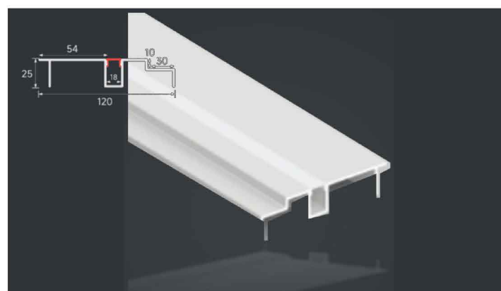
LSH-120 Double-Step Double-step ceiling profile Diffuser: PC cover
