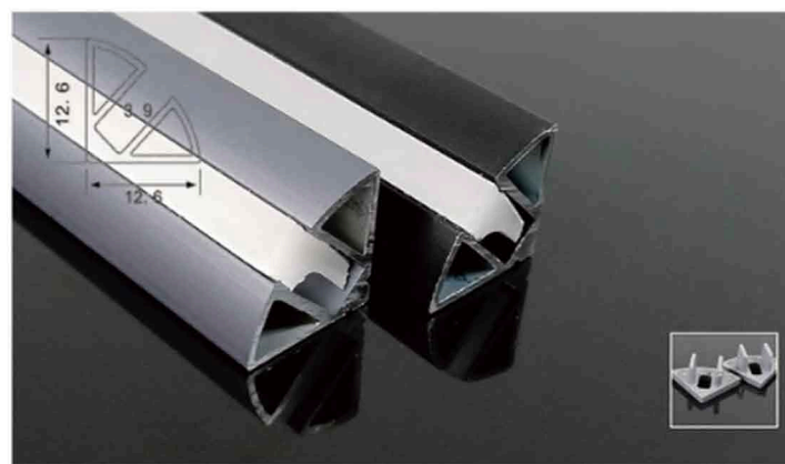
LSH006 13x13mm Color: Black/White/Silver Diffuser Cover: Clear/Frost/Opal/Black
