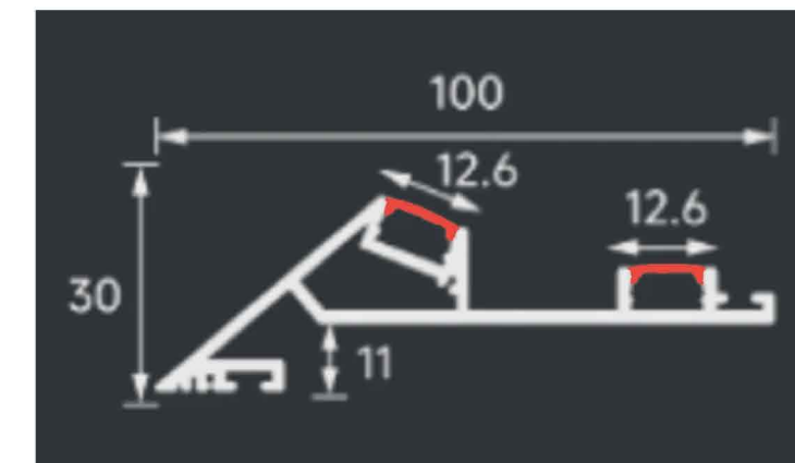
LSH-10030 Slim Flange
