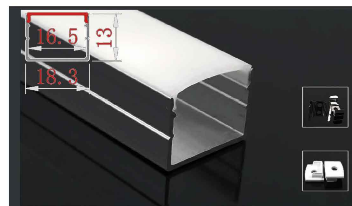
XT-340 Compact Linear Housing Cover & finish: Specify with order
