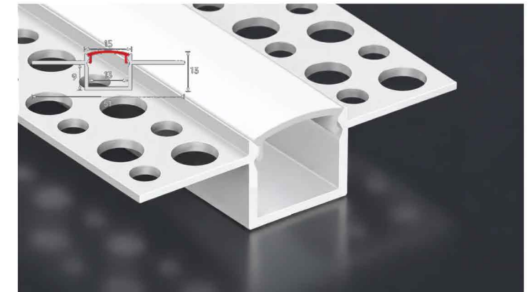
LSH-1513DU Double-wing plaster-in Cover & finish: Confirm by model
