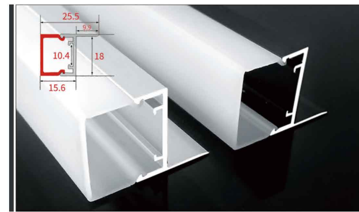
GD-010 Color: Black / White / Silver PC Cover: Opal / Frost
