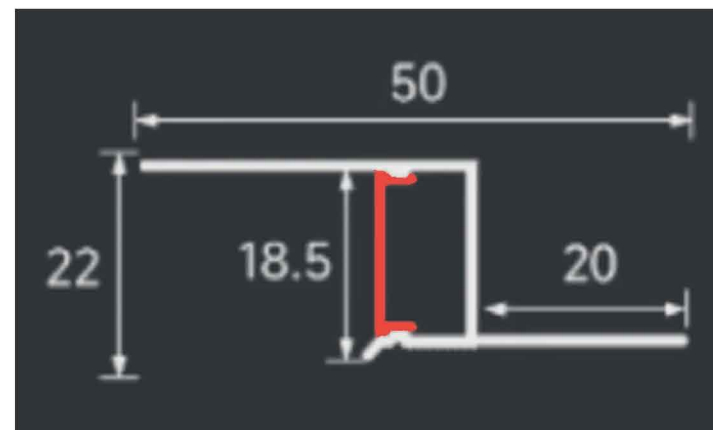
LSH-5020 Lower Flange
