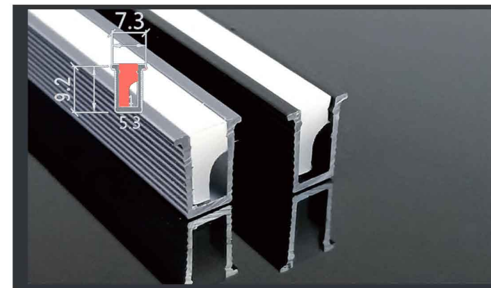
GD-004 Finish: Silver Diffuser: Clear / Opal / Frost / Black
