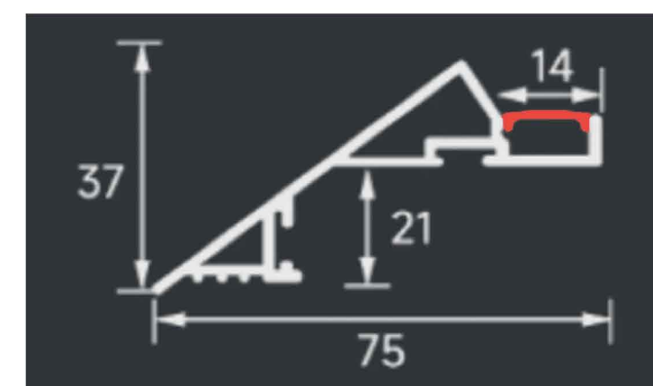
LSH-7537 Slim Flange
