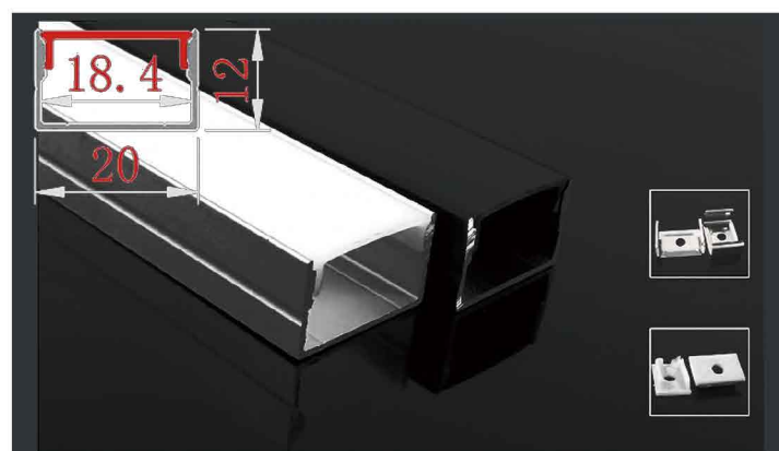
XT-308 Rectangular Strip Channel Cover & finish: Specify with order
