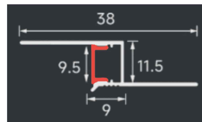
LSH-3814 Lower Flange
