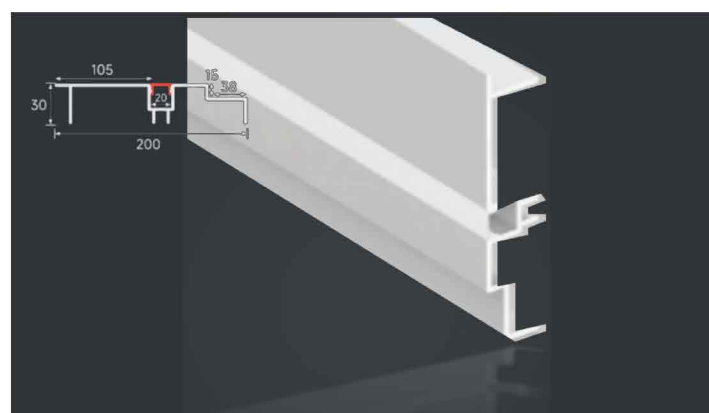
LSH-200 Double-Step Double-step ceiling profile Diffuser: PC cover
